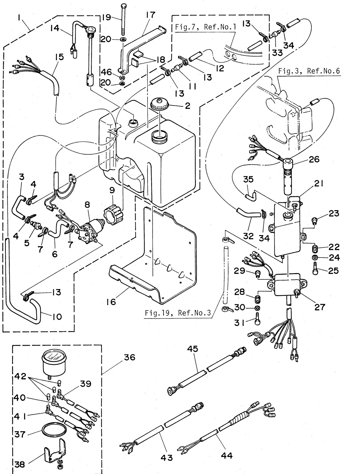
Fig. 20 OIL TANK
