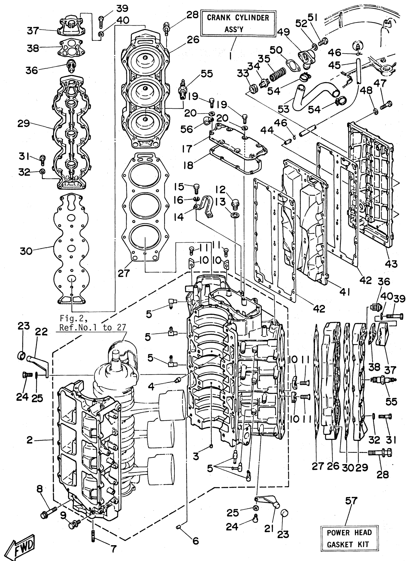
Fig. 1 CRANKCASE & CYLINDER
