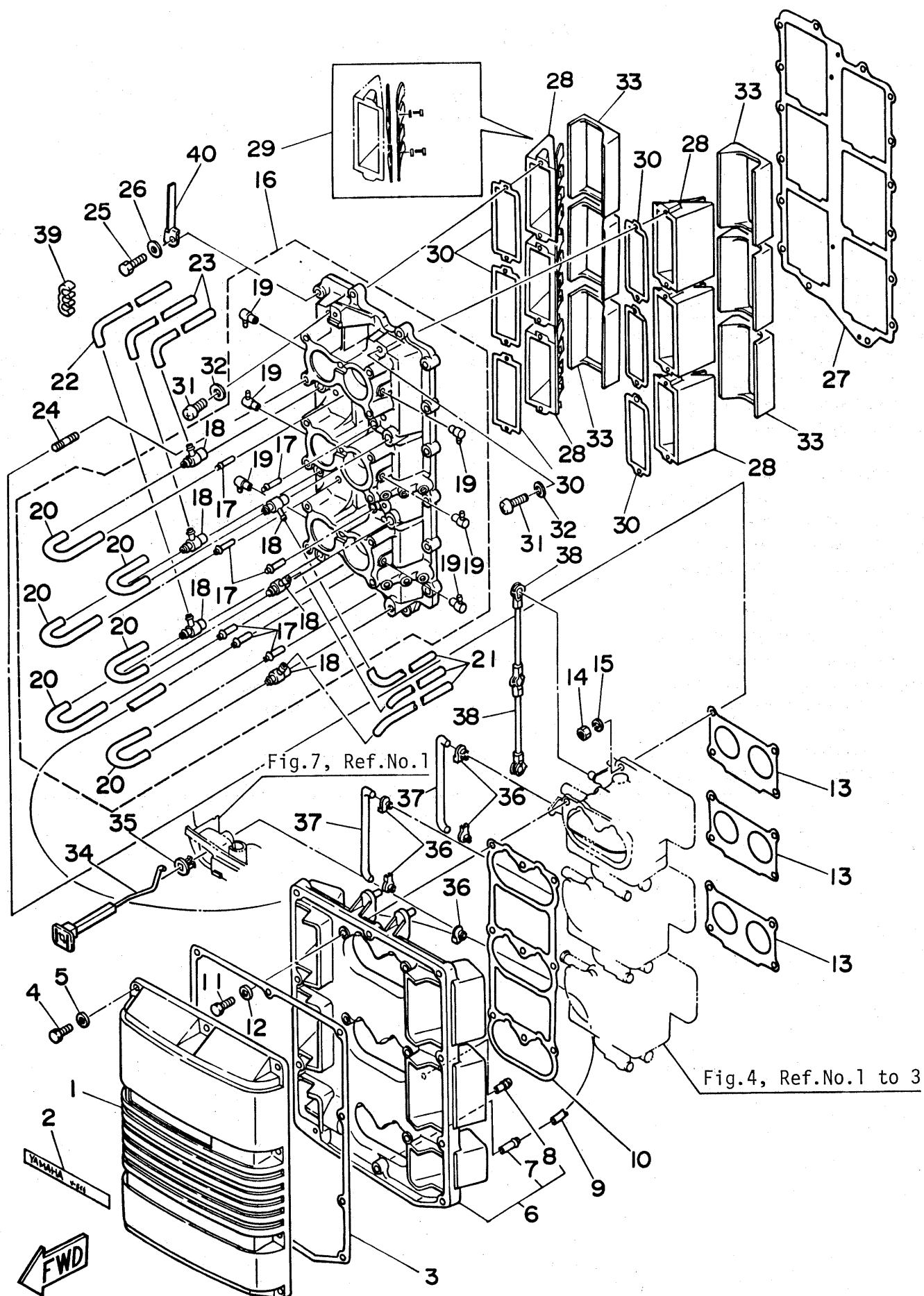
Fig. 3 INTAKE
