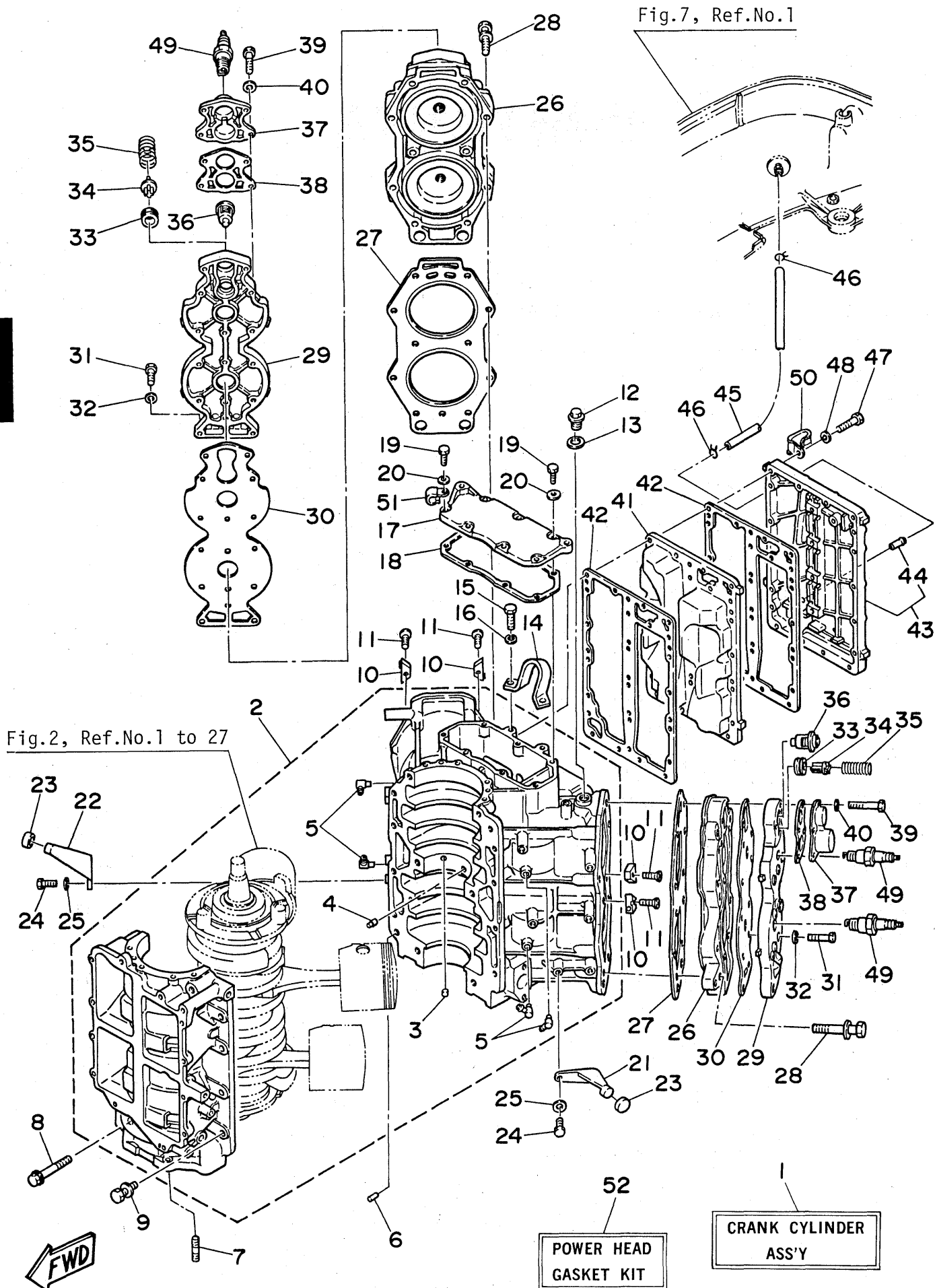
Fig. 1 CRANKCASE & CYLINDER
