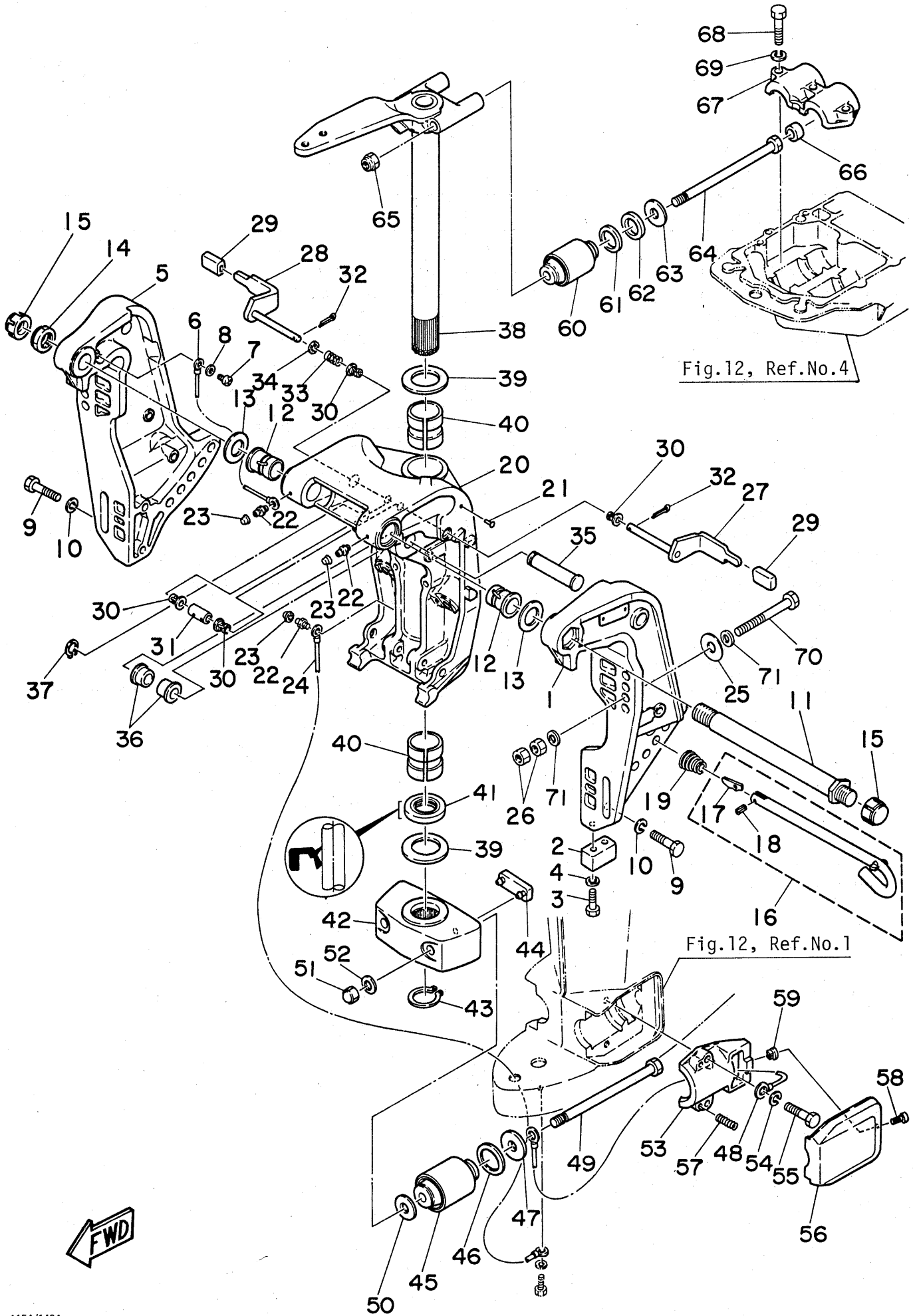
Fig. 8 BRACKET 1
