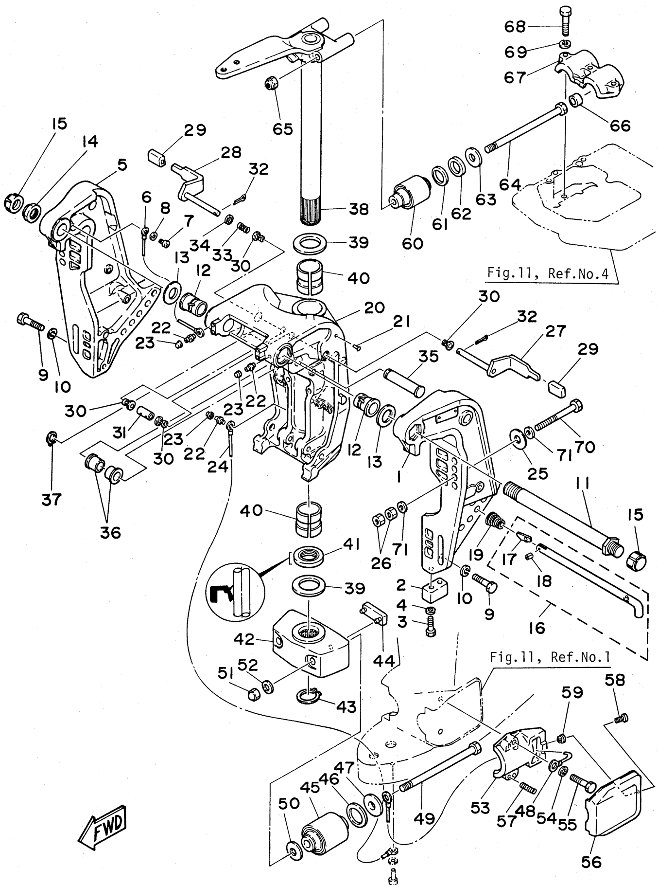
Fig. 8 BRACKET
